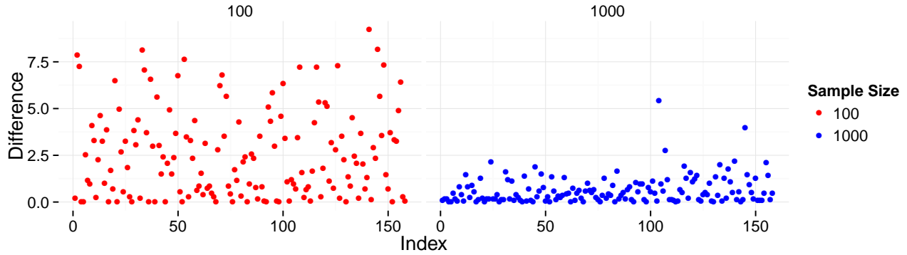
Fig. 4. The difference from true mutation score when sample size is 100, and when sample size is 1,000 in %. The projects are ordered by the total number of mutants, which shows that accuracy has no relation to project size.
