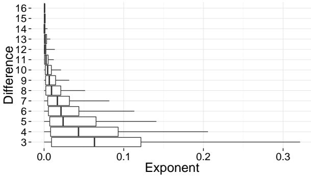
Fig. 3. This graph shows the progressive improvement of accuracy ( x ) as sample sizes increase as powers of 2 ( 2^i ) for 158 projects. The boxes in boxplots represent 0.25 and 0.75 quantiles, and the ends of black lines represent quantiles at 0.025 and 0.975 respectively. This figure shows how precision improves as sample size increases.
