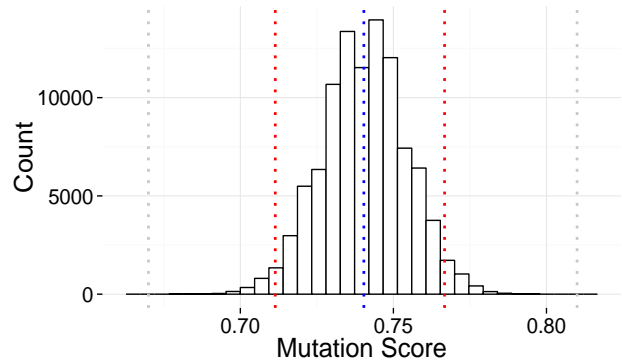
Fig. 2. The distribution of mean mutation score when sample size is 1,000 for Apache commons-math. The central blue line shows true mean at 74.03, and the red lines mark 95% confidence intervals. Similarly the gray lines show the theoretical bounds for 95% confidence intervals. This shows that the sample variation is well within theoretical bounds.
